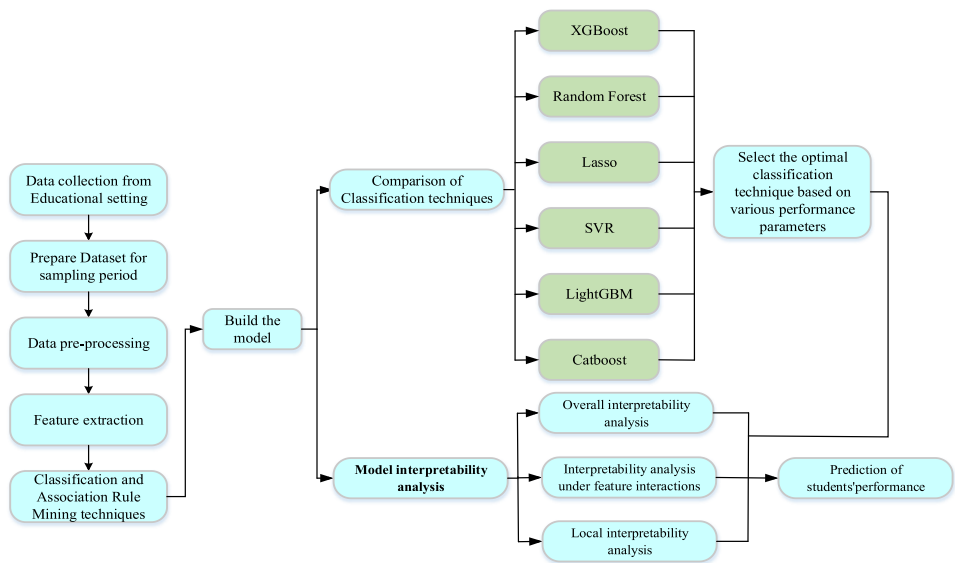
Fig. 1. Data mining process to predict students' performance.
