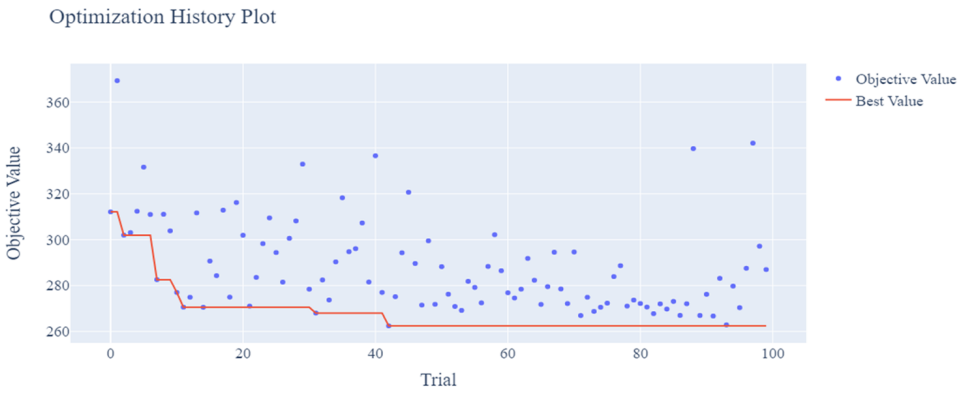
Fig. 5. Parameter optimization process of XGBoost algorithm.
