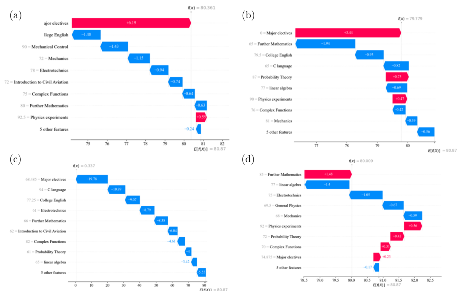
Fig. 9. Local interpretability of SHAP values for samples. (a) Local interpretability of SHAP values for sample A. (b) Local interpretability of SHAP values for sample B. (c) Local interpretability of SHAP values for sample C. (d) Local interpretability of SHAP values for sample D.
