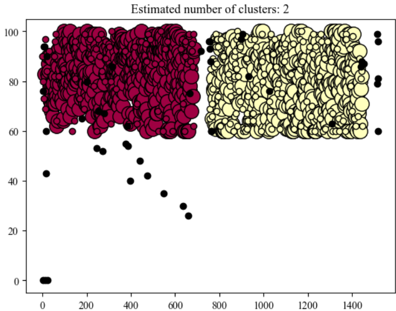
Fig. 3. Clustering results of DBSCAN algorithm.
