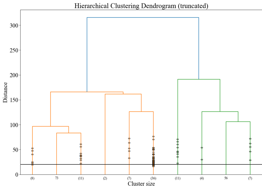
Fig. 2. Clustering results of academic performance classification for fresh graduates.
